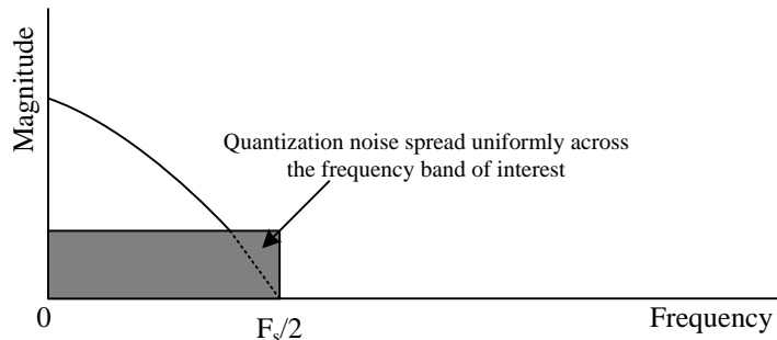
(a) Sampling at Nyquist rate
