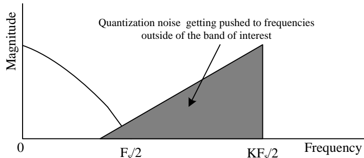
(b) Oversampling with a factor k results in the quantization noise being pushed out towards KF_s/2
